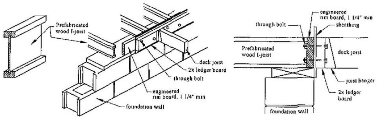
Figure 8: Deck attachment to engineered rim board
