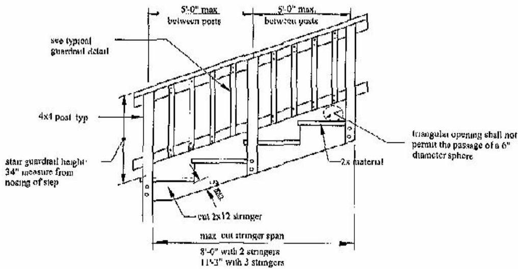
Figure 23: Guardrail and cut stringer detail
