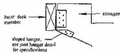
Figure 28: Stair connection requirements
