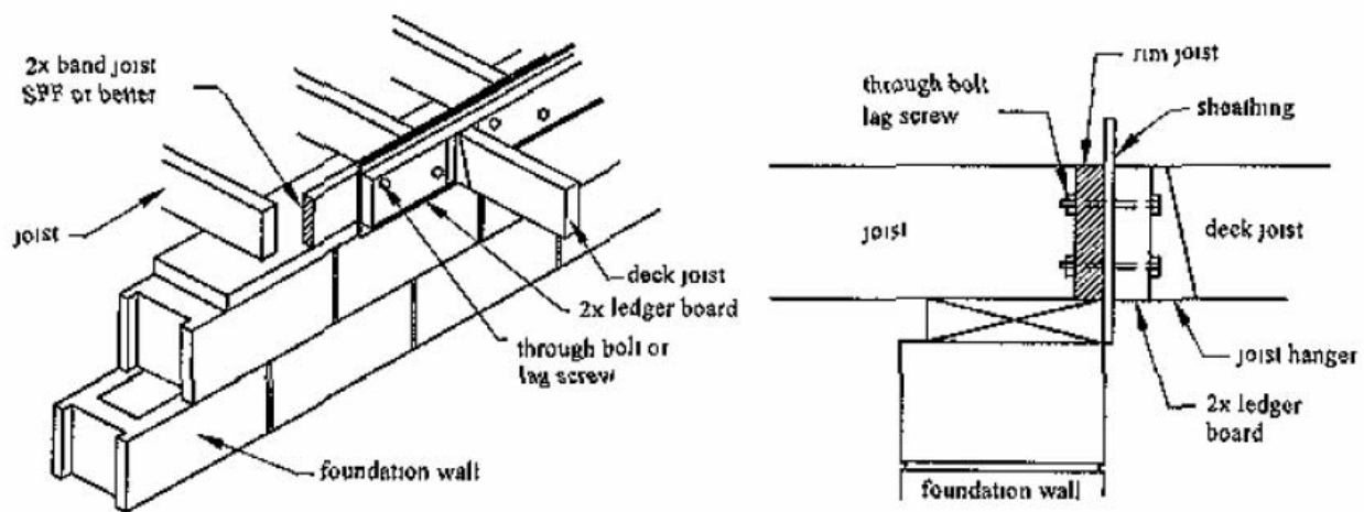
Figure 7: Deck attachment to single dimensional band joist
