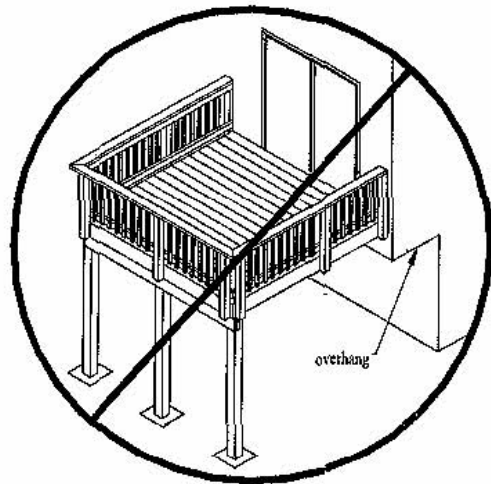
Figure 12: Attachment to house overhang is prohibited
