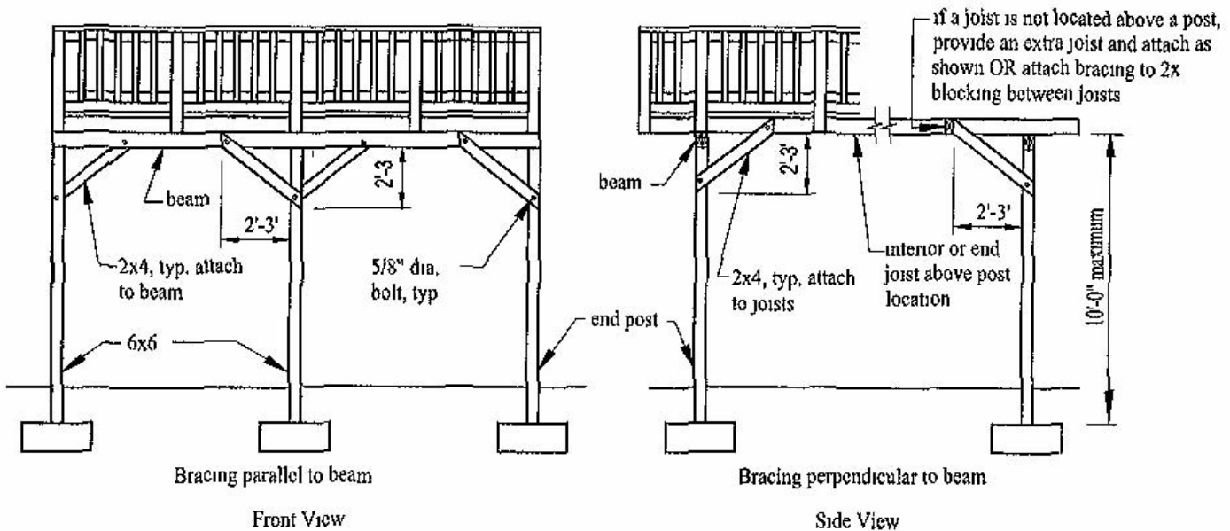
Figure 15: Bracing for freestanding decks
