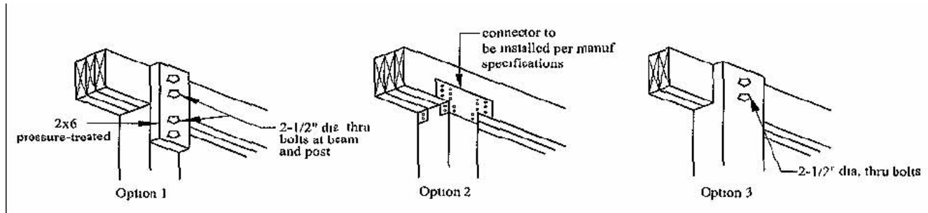
Figure 21: 6x6 inches post-to-beam connection
