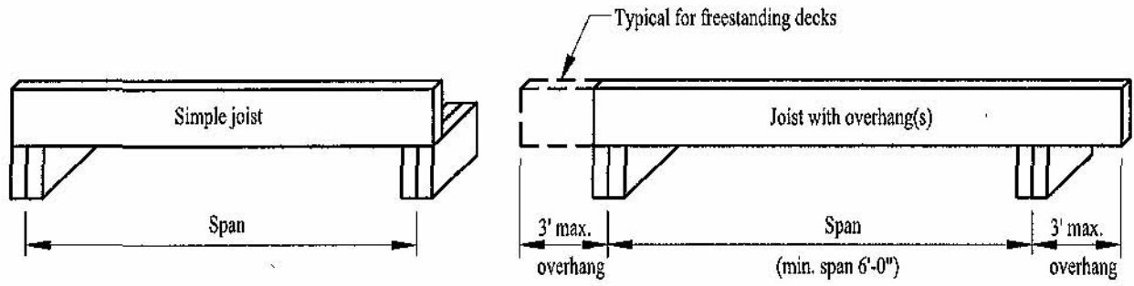
Figure 2: Joist Span Types
