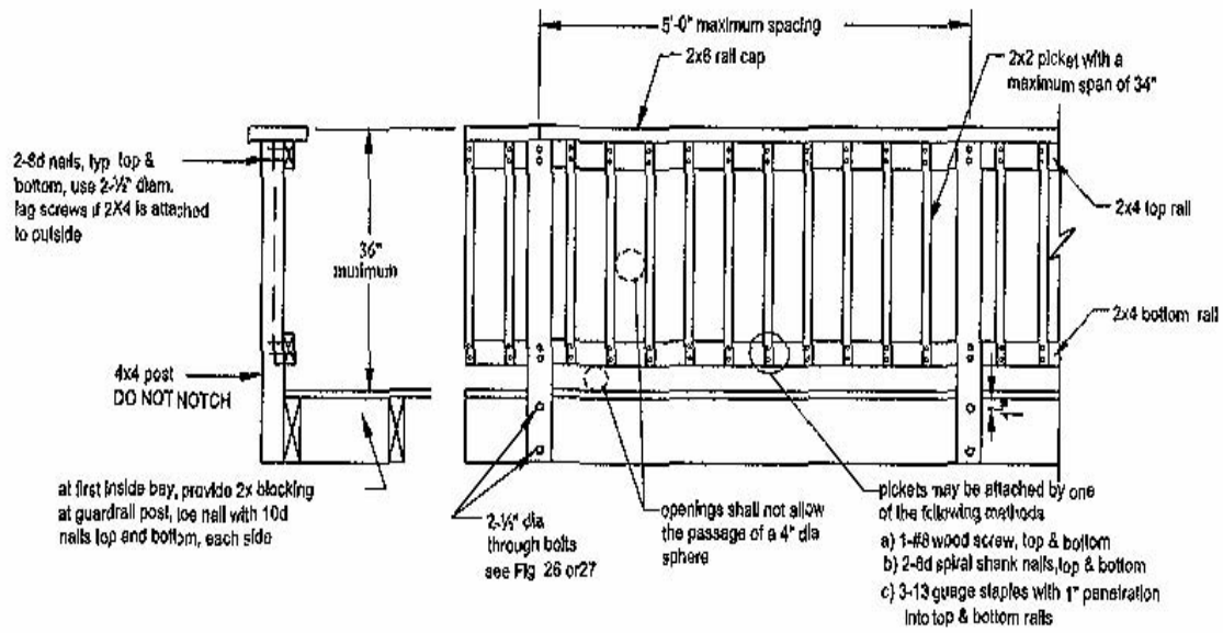
Figure 22: Typical guardrail details
