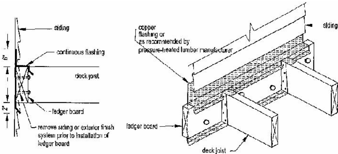
Figure 14: Flashing requirements
