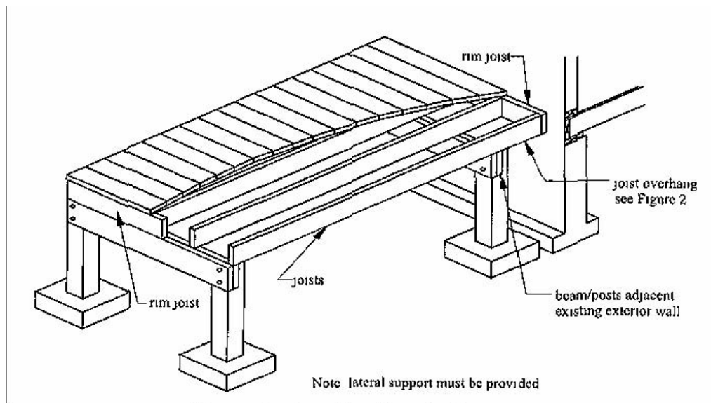
Figure 6: Freestanding deck
