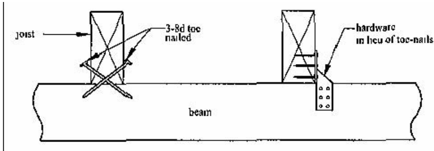
Figure 16: Joist to beam detail
