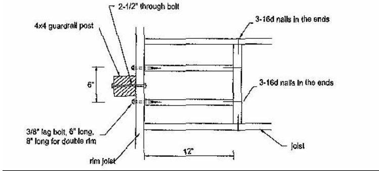
Figure 24: Plan (top) view-Exterior guardrail post
