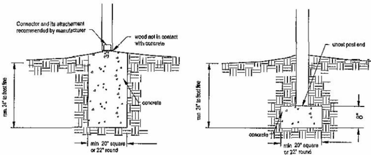
Figure 5: Typical footing details
