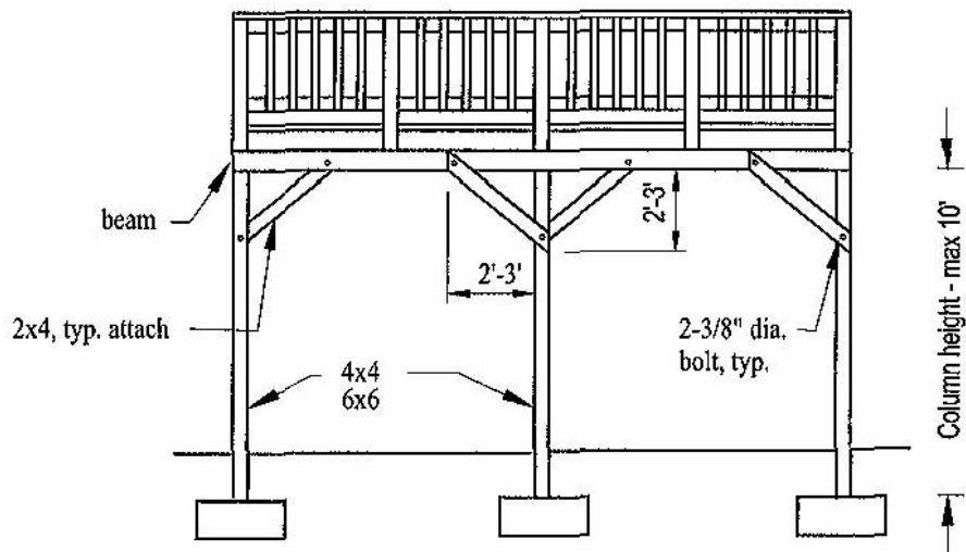
Figure 4: Deck posts
